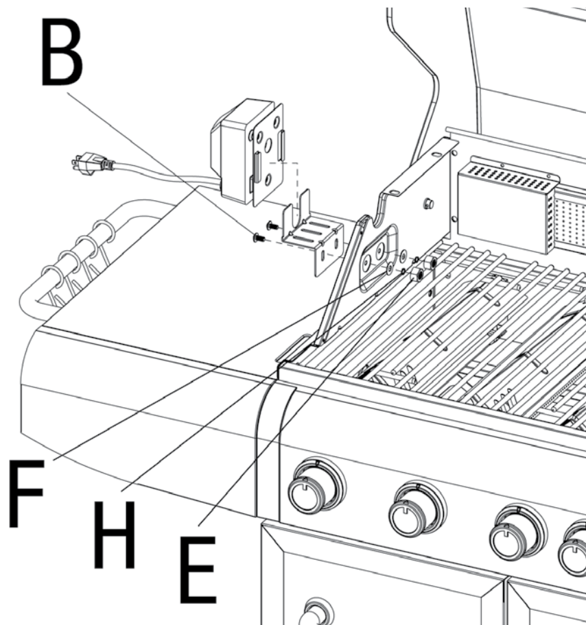
Attach Rotisserie Motor Support and Rotisserie Motor
